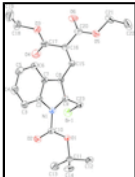
Fig. 1. The molecular structure of the title compound. Displacement ellipsoids are drawn at the 30% probability level. H atoms have been omitted for clarity.
