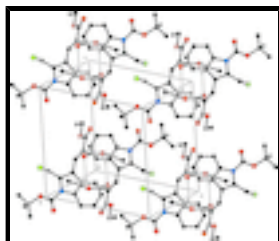
Fig. 2. A view of the crystal packing of molecules, showing C–H...O interactions (dashed lines), leading to dimer formation.
